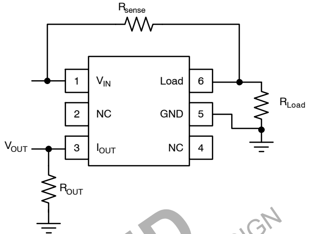
Figure 2. Typical Circuit
