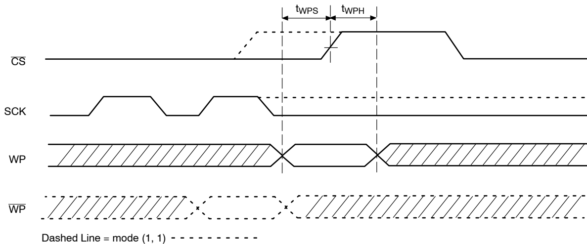
Figure 8. WP Timing
